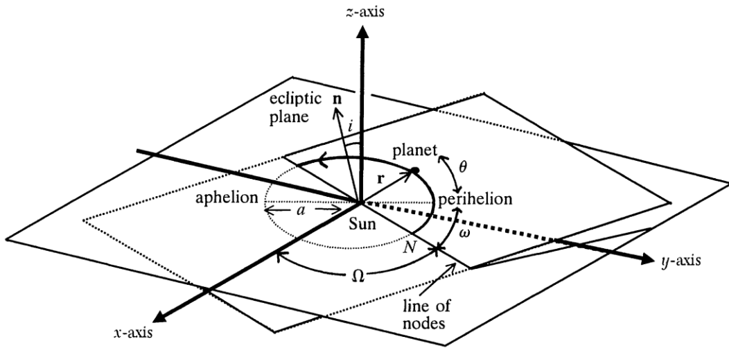
FIGURE 1 Parameters describing the planetary orbit
