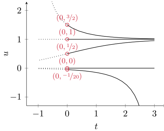
Figure 1.1: Logistic equation — five different trajectories related to the indicated initial conditions with parameters a = 1 , b = 1 , c = 0 .
