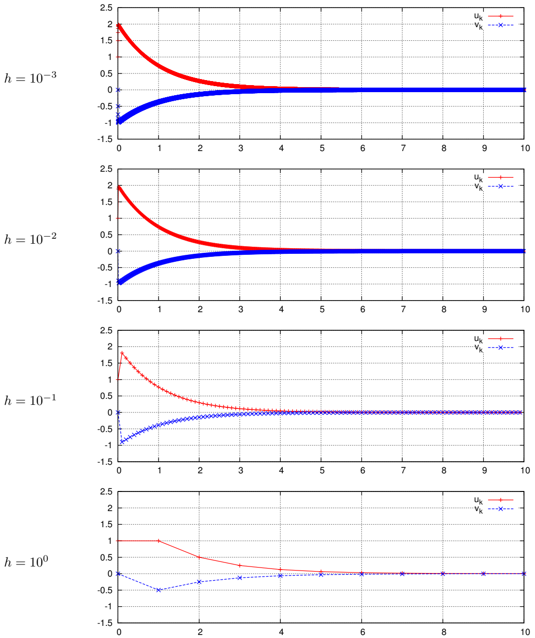
Figure 10.6: Approximate solution of (10.33) by the implicit Euler method.
